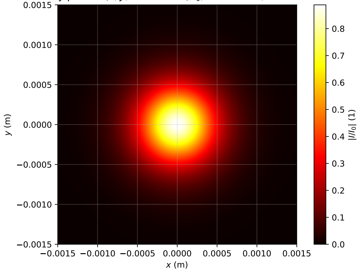
Intensity profile I(x, y, z = 3.901m)/I_0 , P_{in}=0.8P_{cr} , artificial time
